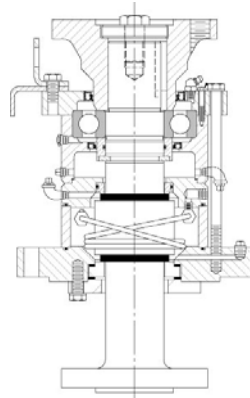
Lightnin cartridge seal with integral bearing.
